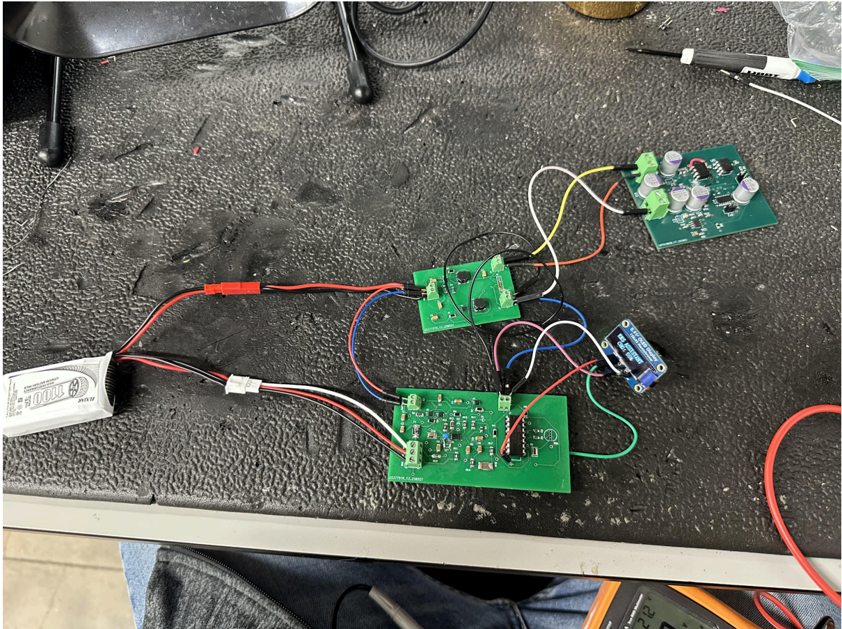
Pre-integration Battery Monitoring, buck converter, and data acquisition boards.
